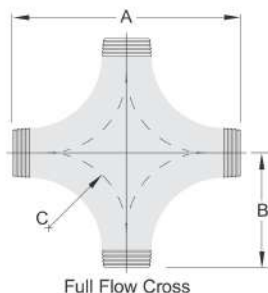
Full Flow Cross
