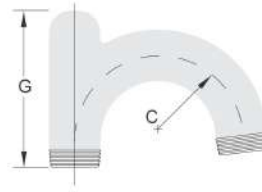
Standpipe Gooseneck With Top Integral Bullplug
